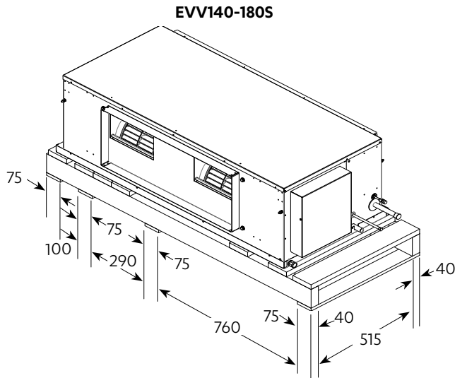
PALLET FORK LIFTING HOLE DIMENSIONS ALL DIMENSIONS IN MM.
