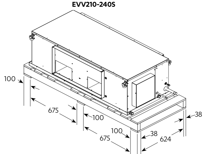
PALLET FORK LIFTING HOLE DIMENSIONS ALL DIMENSIONS IN MM.
