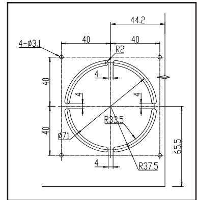
Outside Air Intake Details
