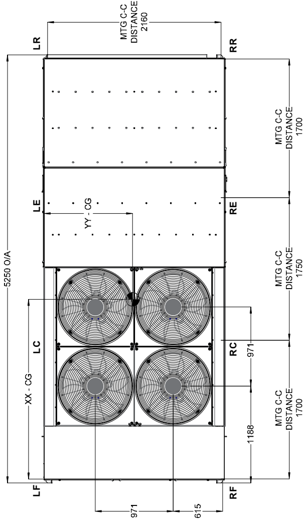
TOP VIEW
