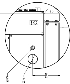
DETAIL A ELECTRICAL ACCESS
